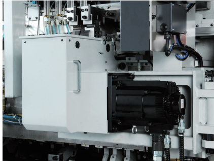
伺服横动加工装置 Servo crossmotion device
